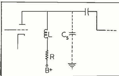
Figure 1 (a) Shunt-compensated video interstage.
