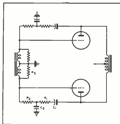
Figure 2 Feedback may be employed around the audio driver stage only as indicated here. Besides reducing distortion, the feedback is used for response control.
